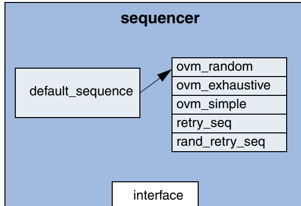
Figure 4-4 Sequencer with a Sequence Library
