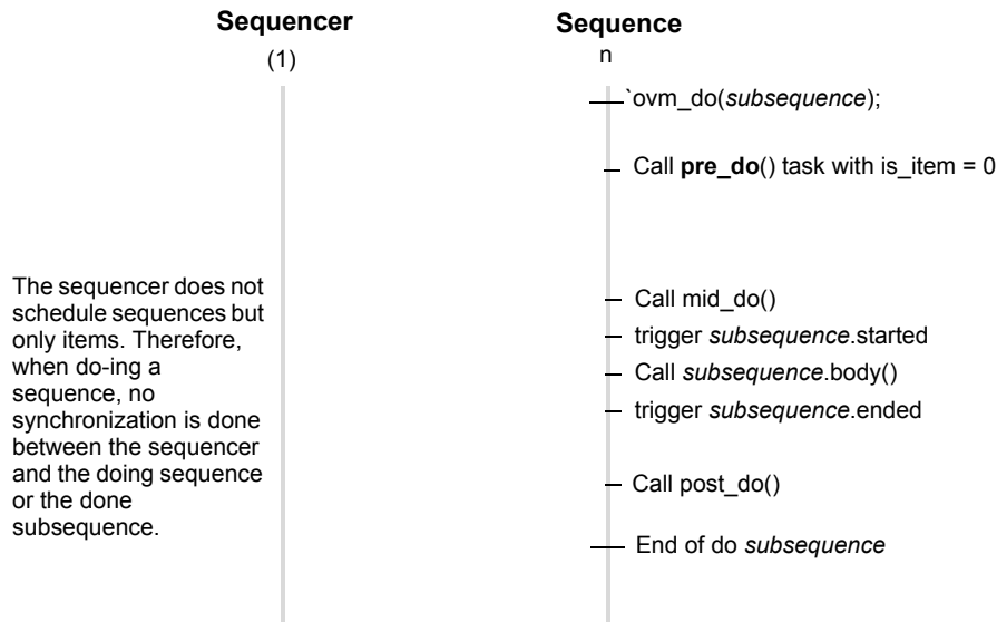
Figure 3-7 Subsequence Flow
