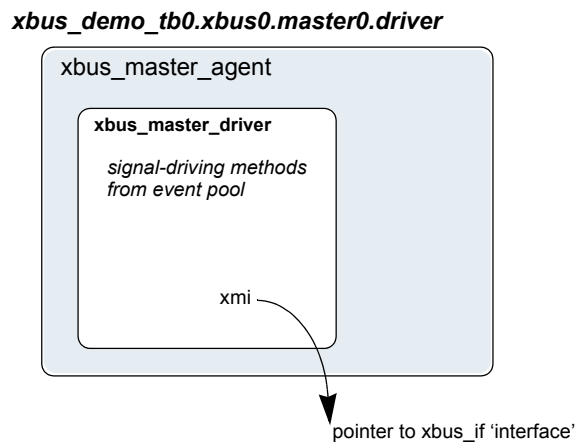
Figure 6-6 Instance of xbus_master_driver
