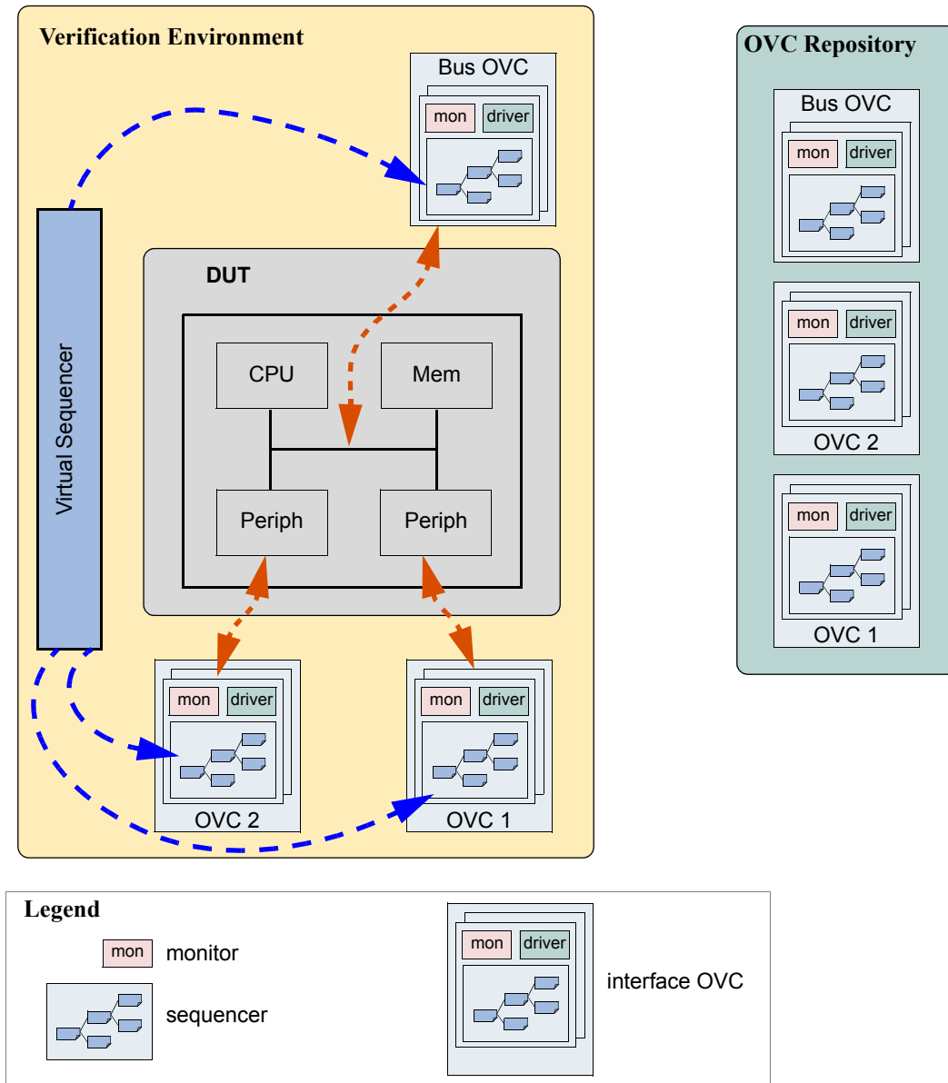
Figure 4-1 Verification Environment Example
