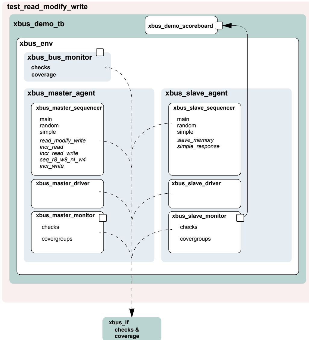
Figure 6-1 XBus Demo Architecture
