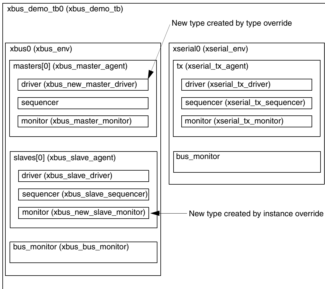
Figure 5-2 Hierarchy Created with Both Overrides Applied
