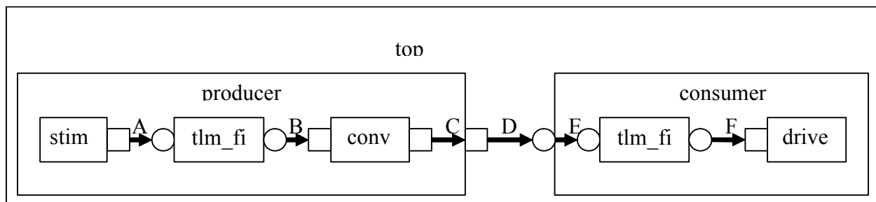
Figure 2-4 Hierarchy in TLM
