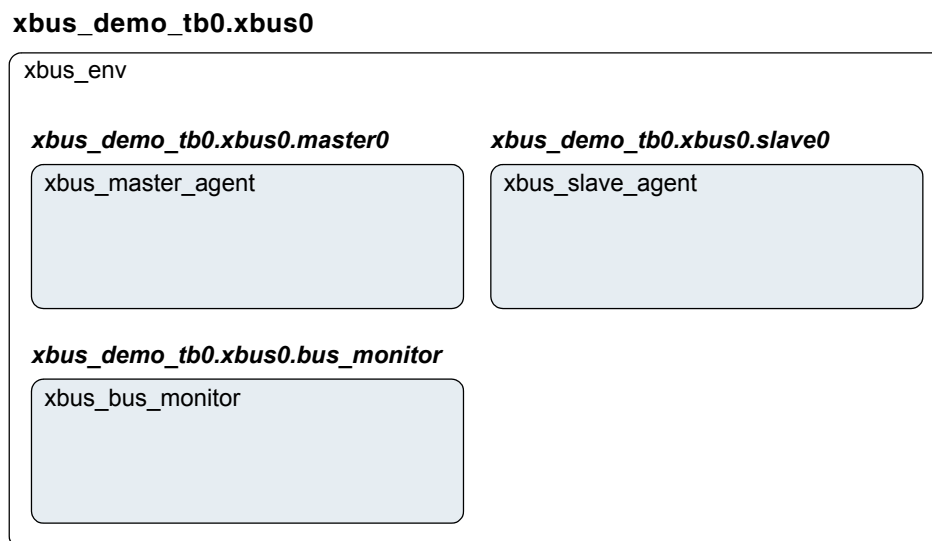
Figure 6-3 Instance of xbus_env
