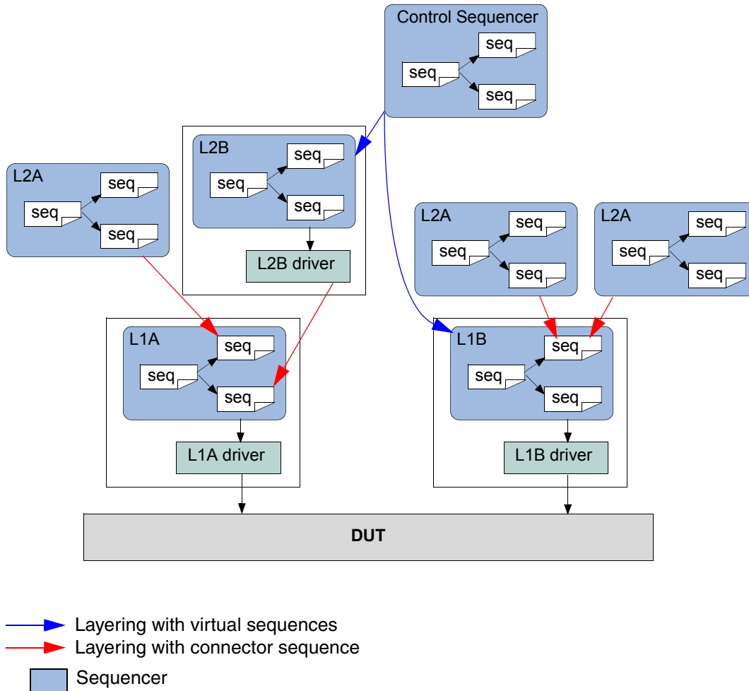
Figure 5-6 Most-General Case of Using Virtual Sequencers
