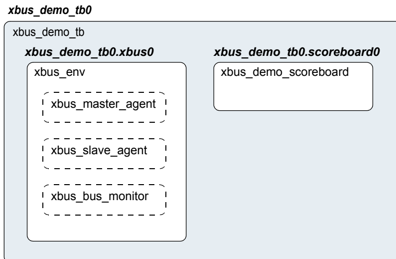
Figure 6-2 Testbench Derived from ovm_env
