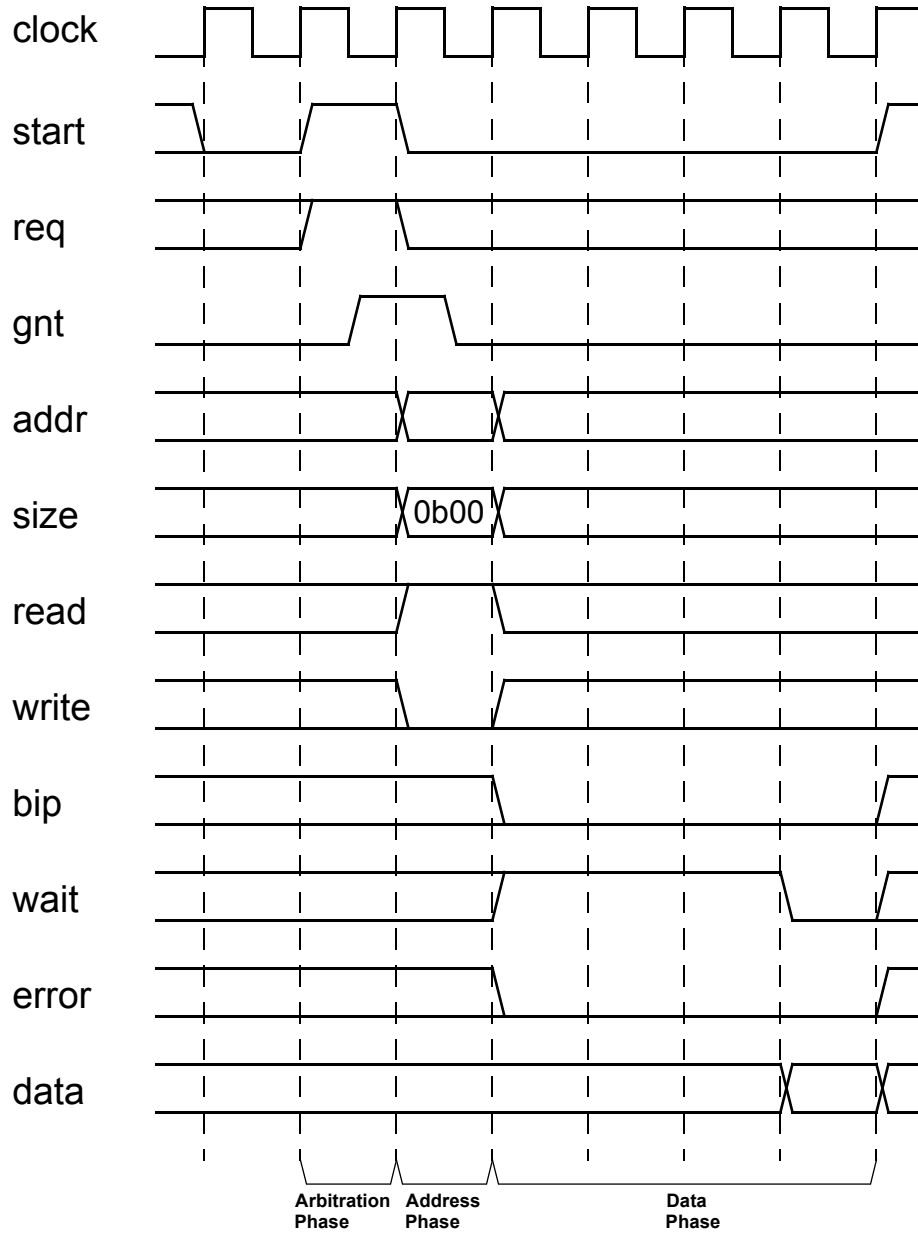
Figure 7-2 Example Read Waveform
