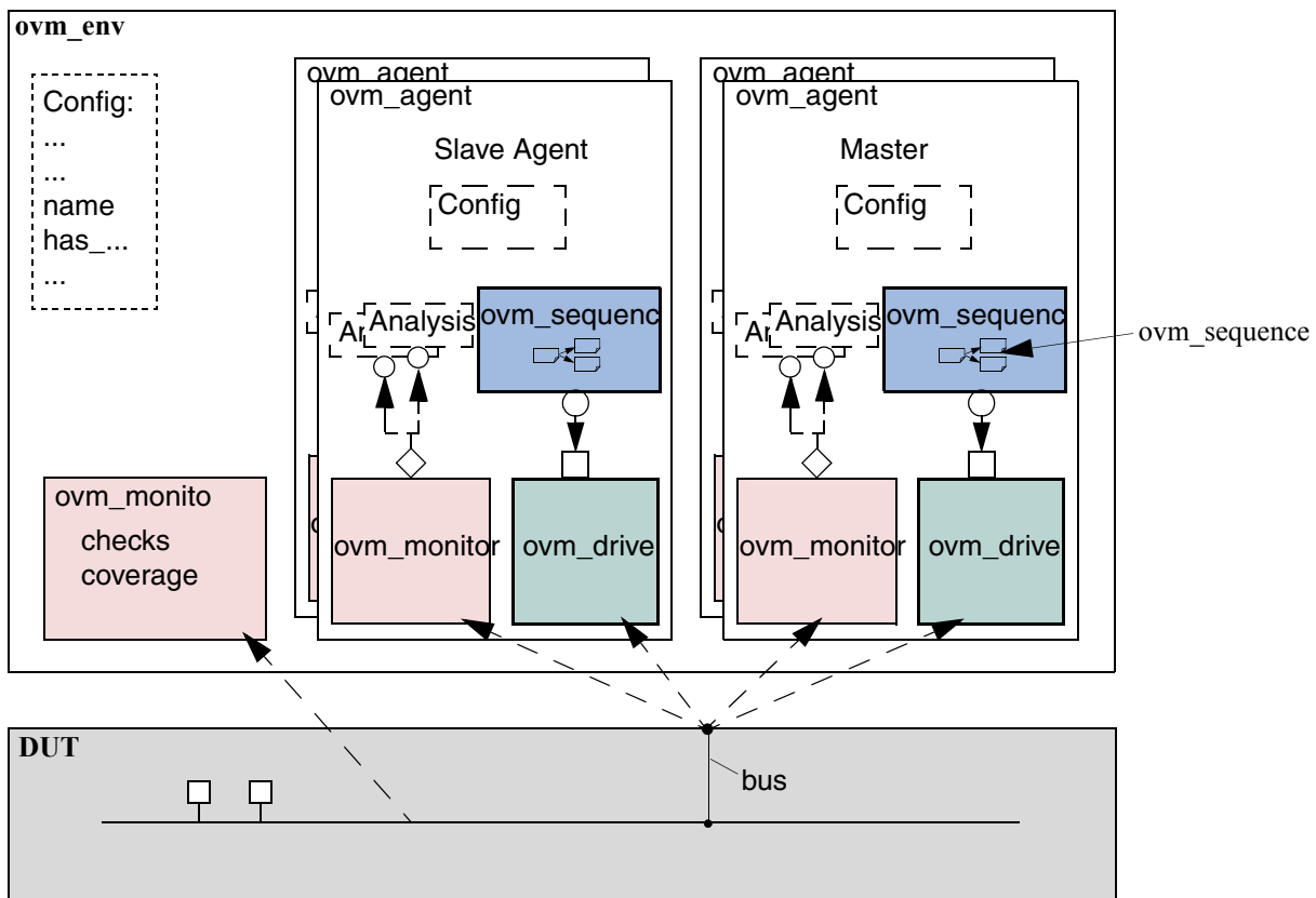
Figure 3-5 Typical OVM Environment Architecture
