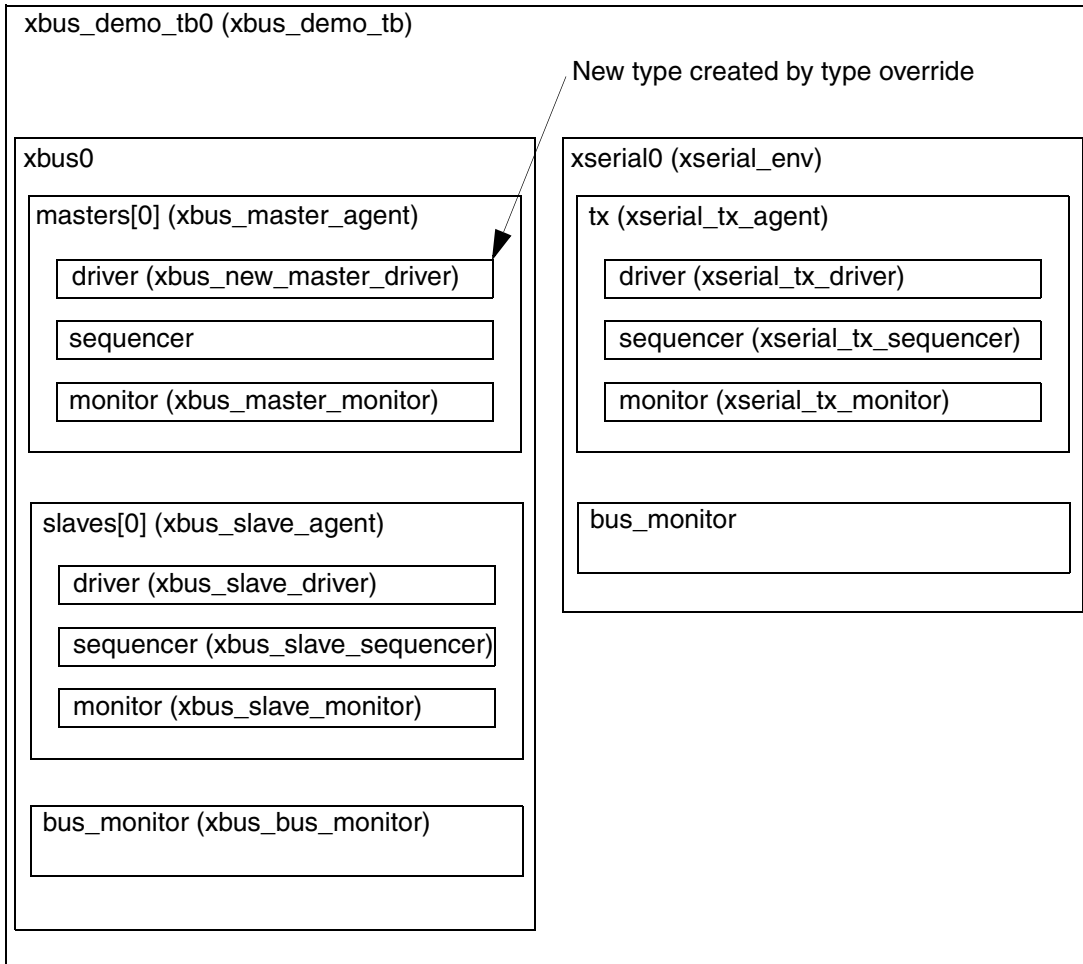
Figure 5-1 Hierarchy Created with set_type_override() Applied
