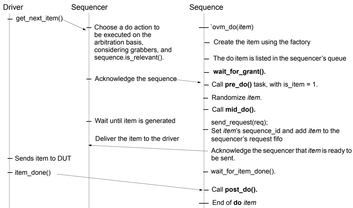
Figure 3-6 Sequence Item Flow in Pull Mode
