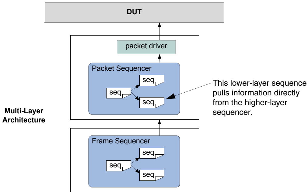
Figure 5-3 Layering Architecture
