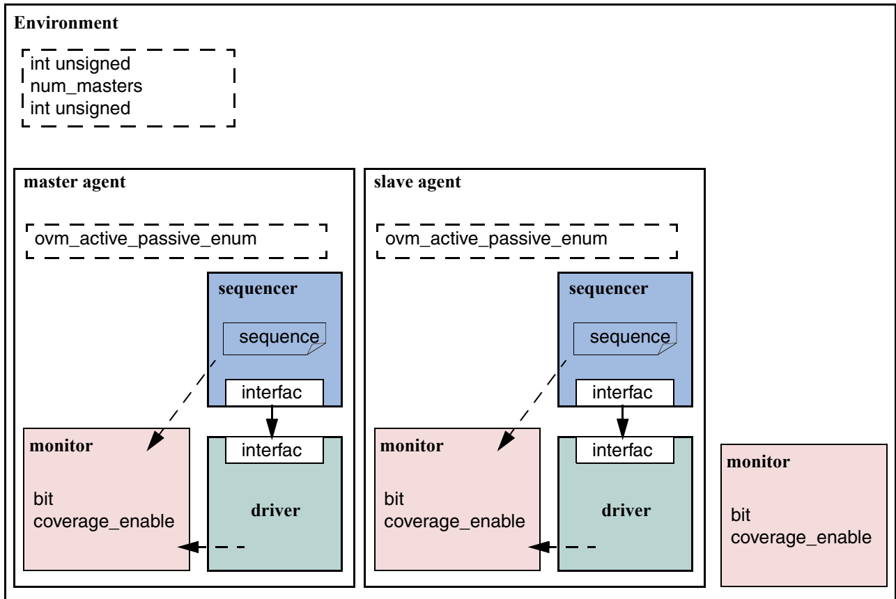
Figure 4-3 Standard Configuration Fields and Locations
