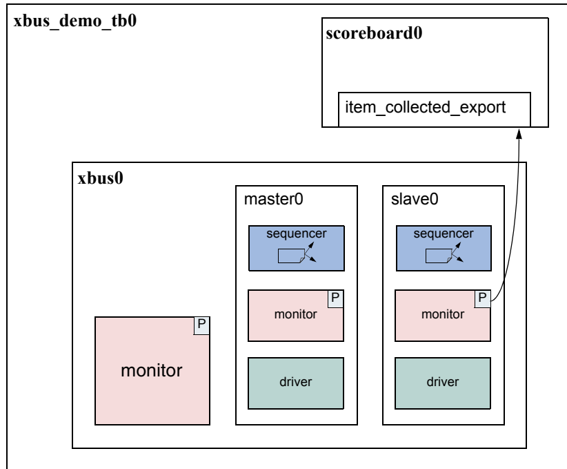
Figure 4-6 XBus Demo Environment
