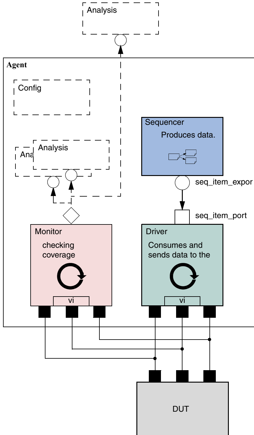
Figure 3-2 Highly Reusable OVC Agent
