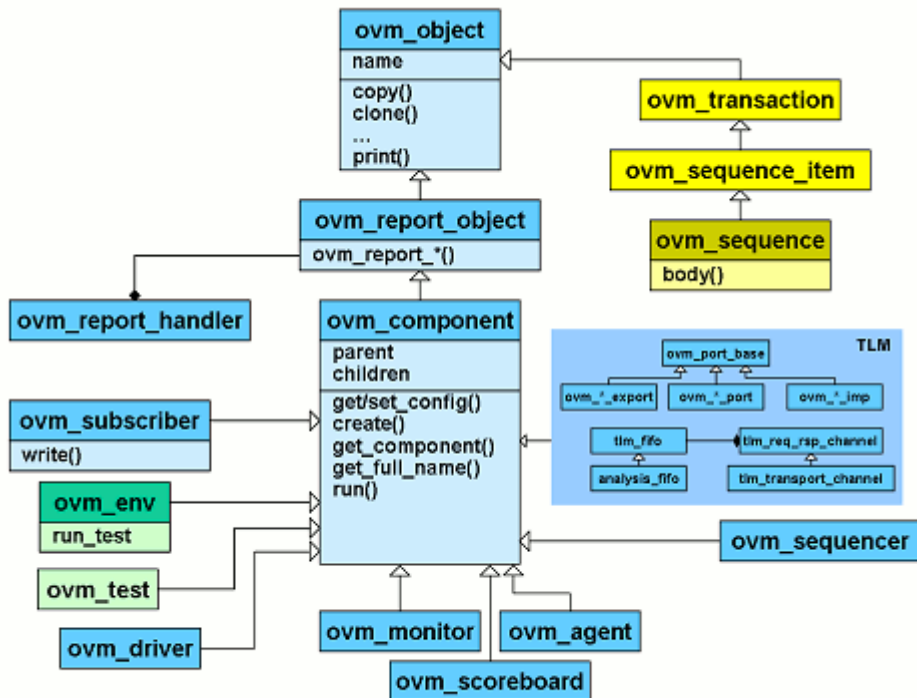
Figure 1-3 (Partial) OVM Class Hierarchy
