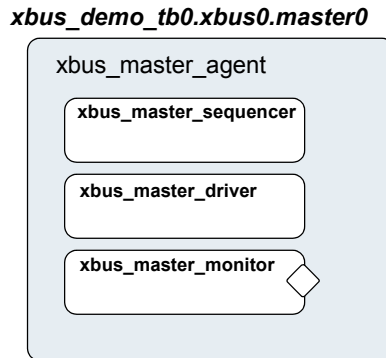
Figure 6-4 Instance of xbus_master_agent
