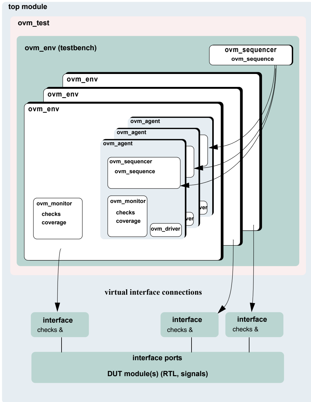
Figure 4-2 OVC Verification Environment Class Diagram
