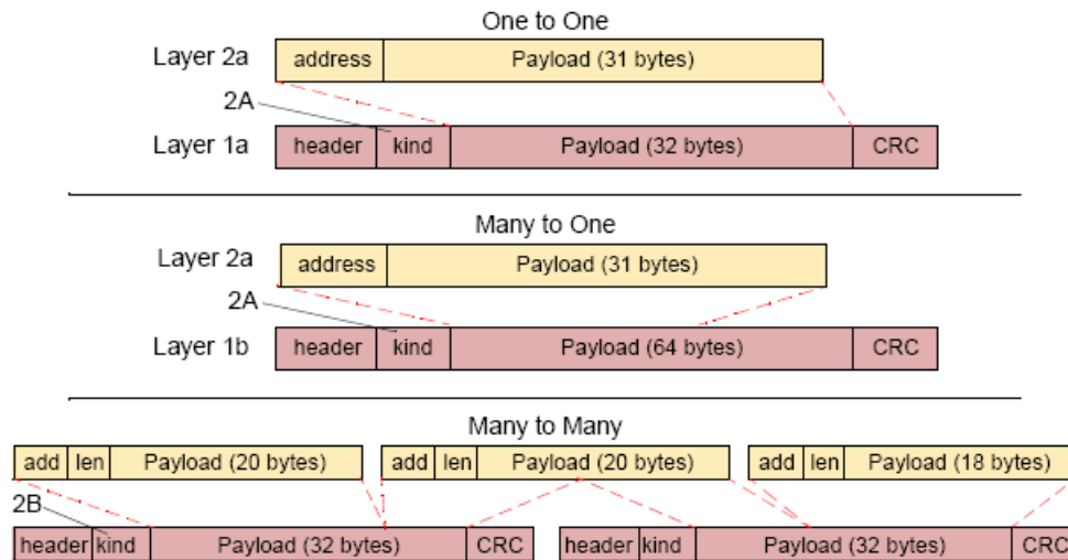
Figure 5-5 Layer Mapping
