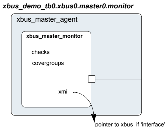
Figure 6-7 Instance of xbus_master_monitor
