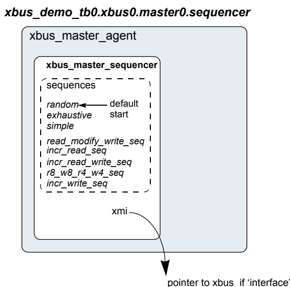
Figure 6-5 Instance of xbus_master_sequencer
