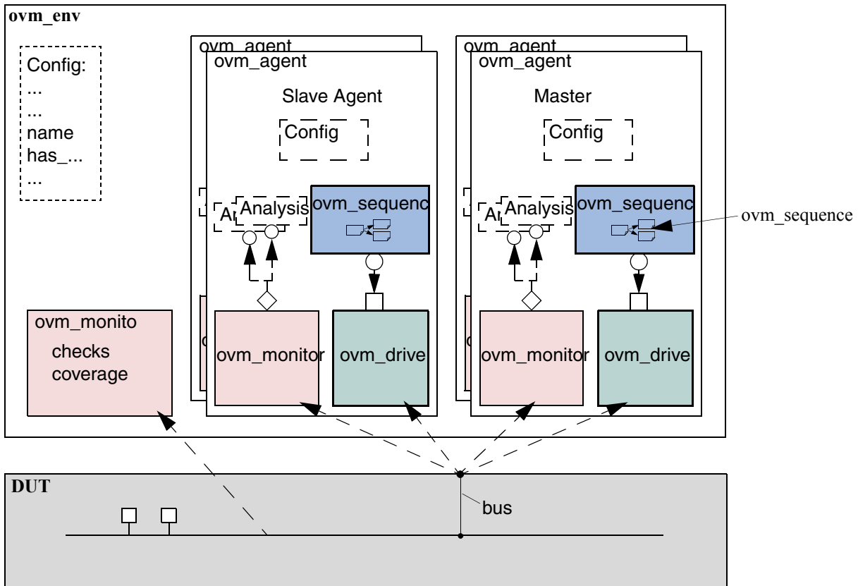
Figure 1-4 Typical OVM Environment Using OVM Library Classes
