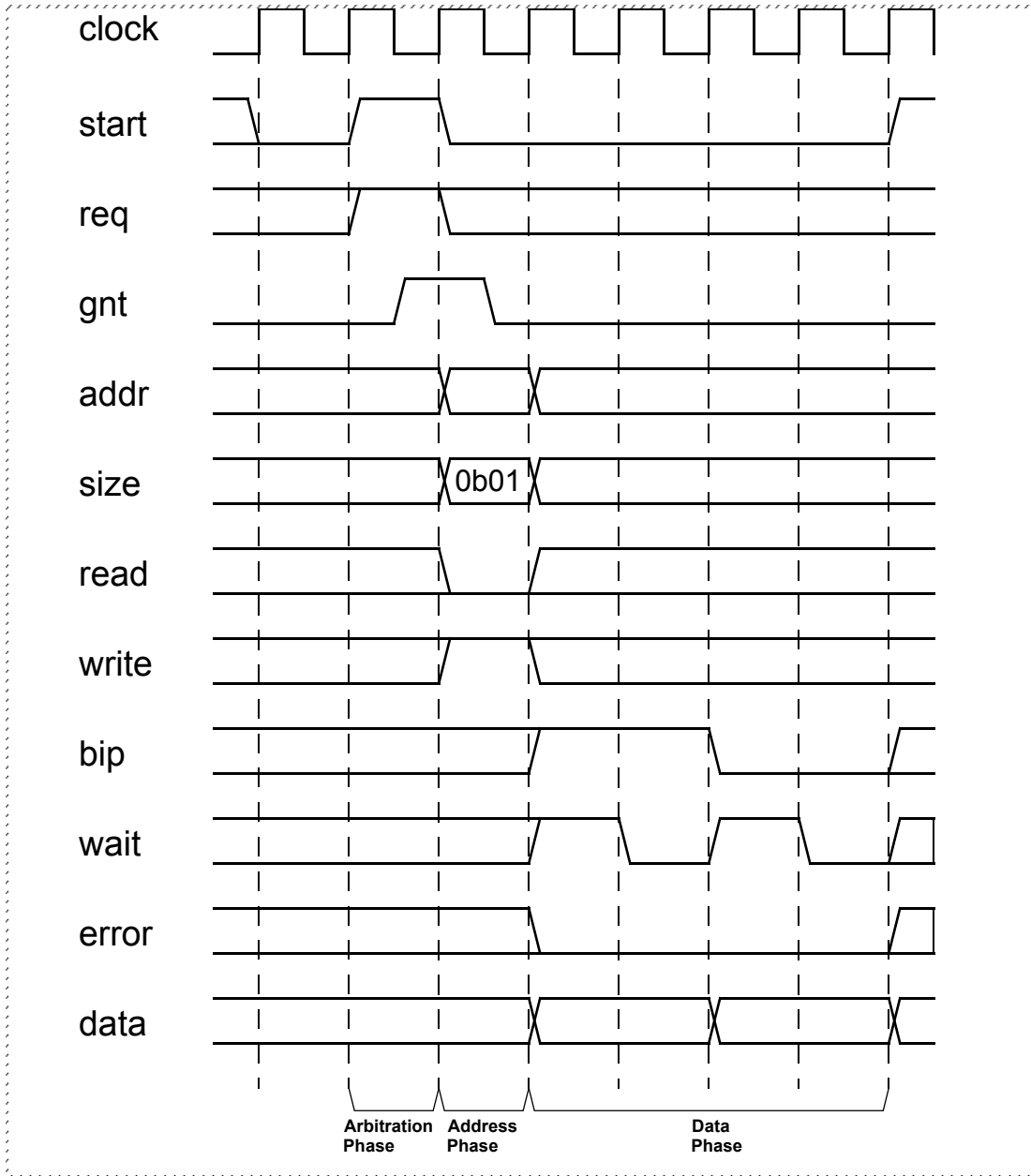
Figure 7-1 Example Write Waveform
