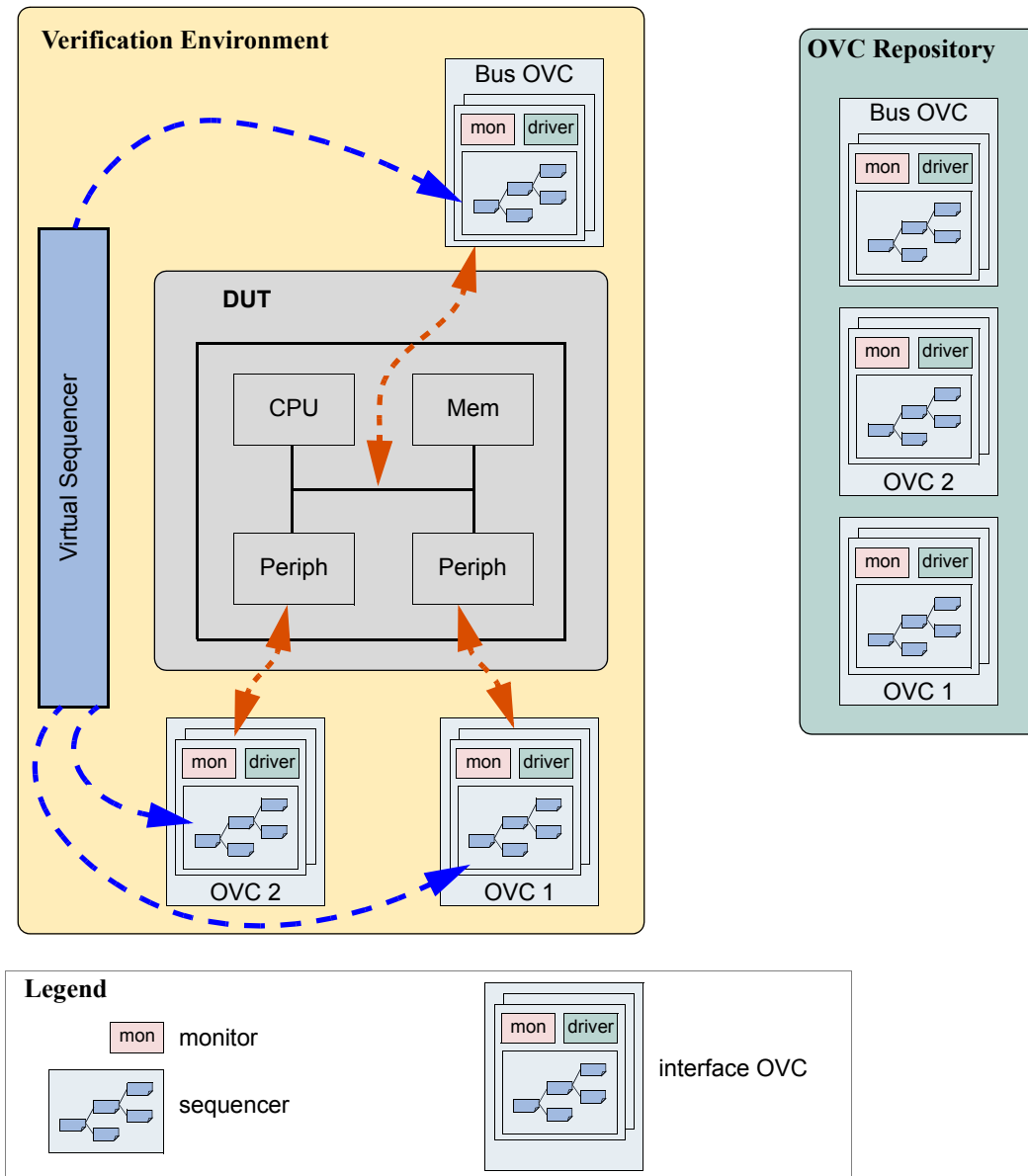
Figure 1-1 Verification Environment Example
