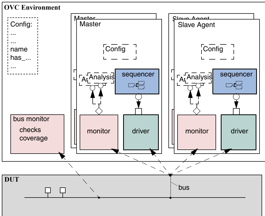
Figure 1-2 Typical OVC Environment
